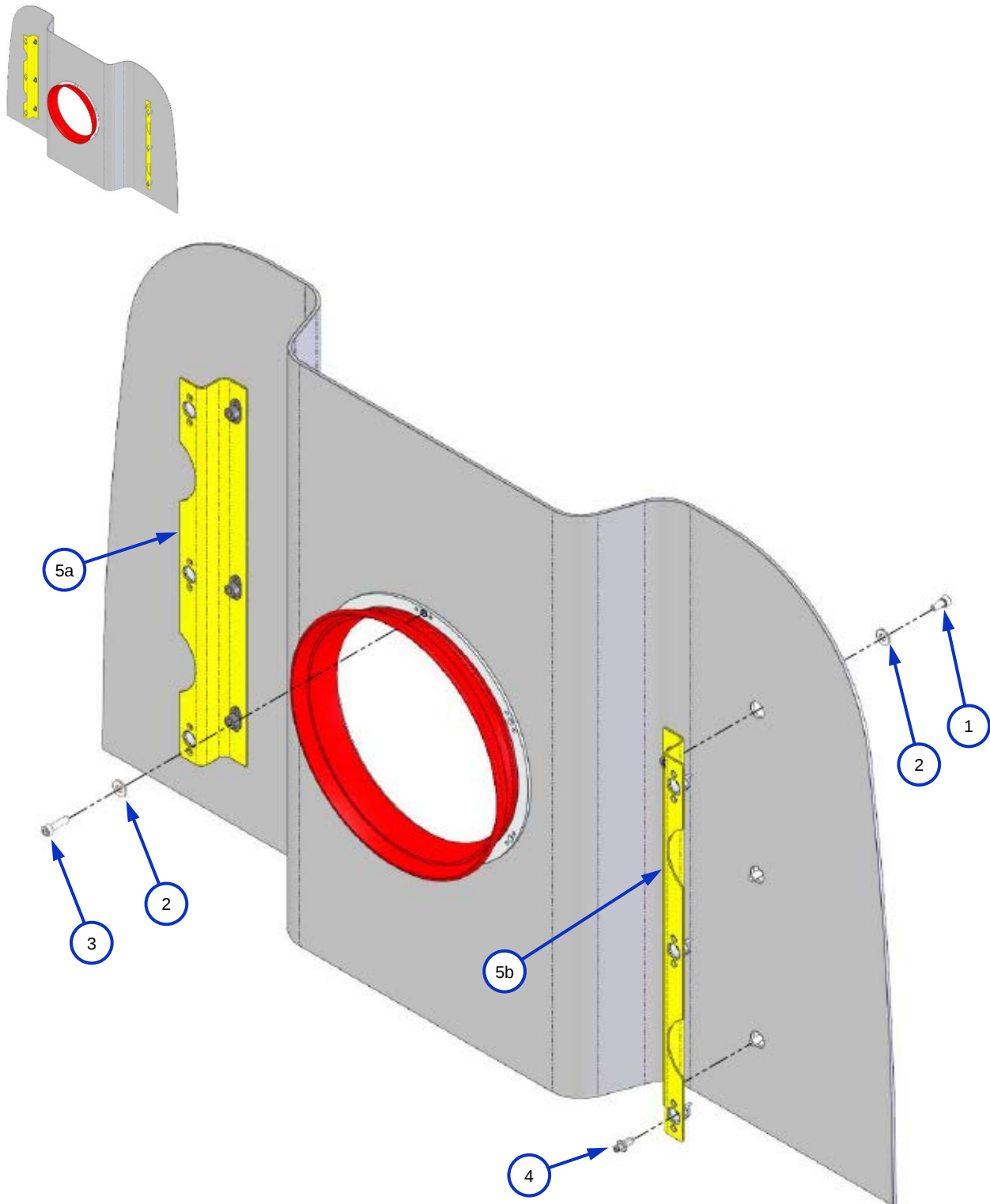
Figure 2-1: FIREWALL MOUNT ASSEMBLY
