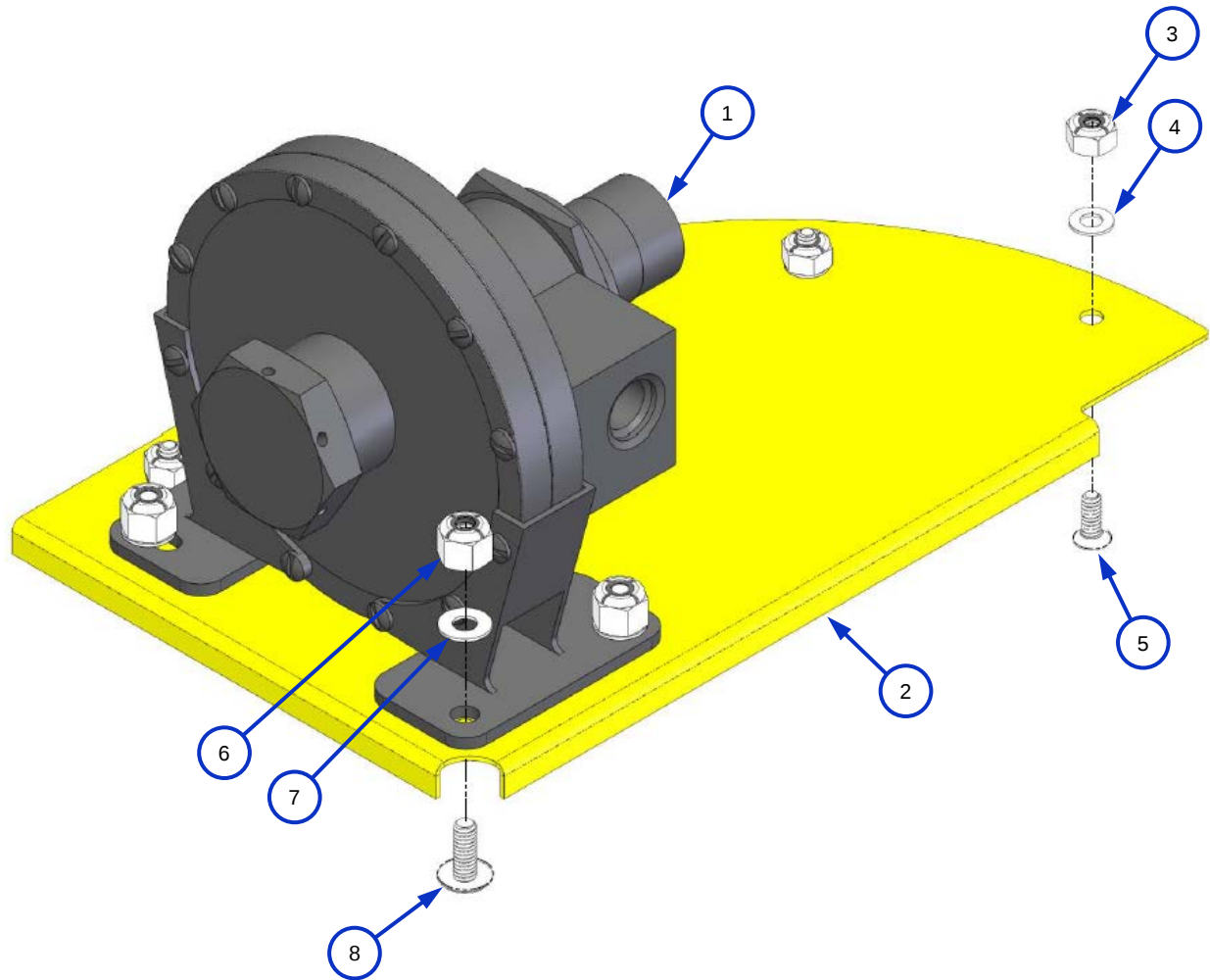
Figure 4-1: DPS INSTALLATION
