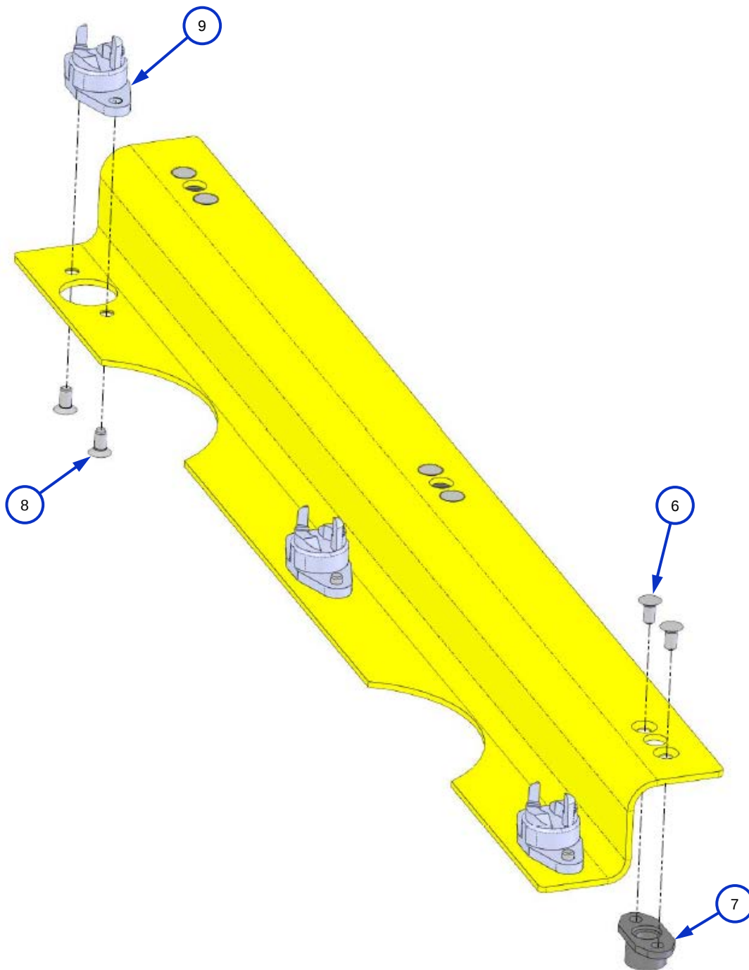
Figure 2-2: MOUNTING BRACKET ASSY, 1206A6-270L/R
