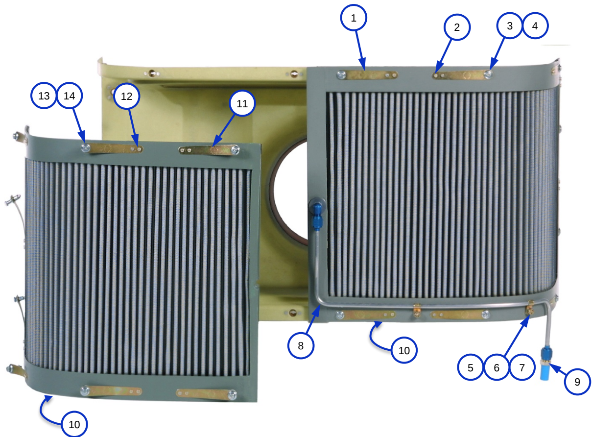
Figure 3-1: FILTER ELEMENT ASSEMBLIES
