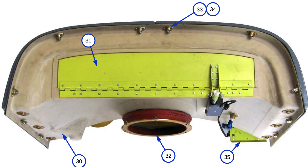
Figure 2-4: MAIN FILTER SYSTEM ASSY TOP VIEW
