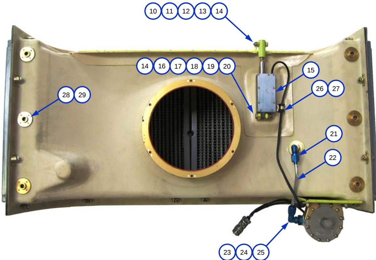
Figure 2-3: MAIN FILTER SYSTEM ASSY FRONT VIEW
