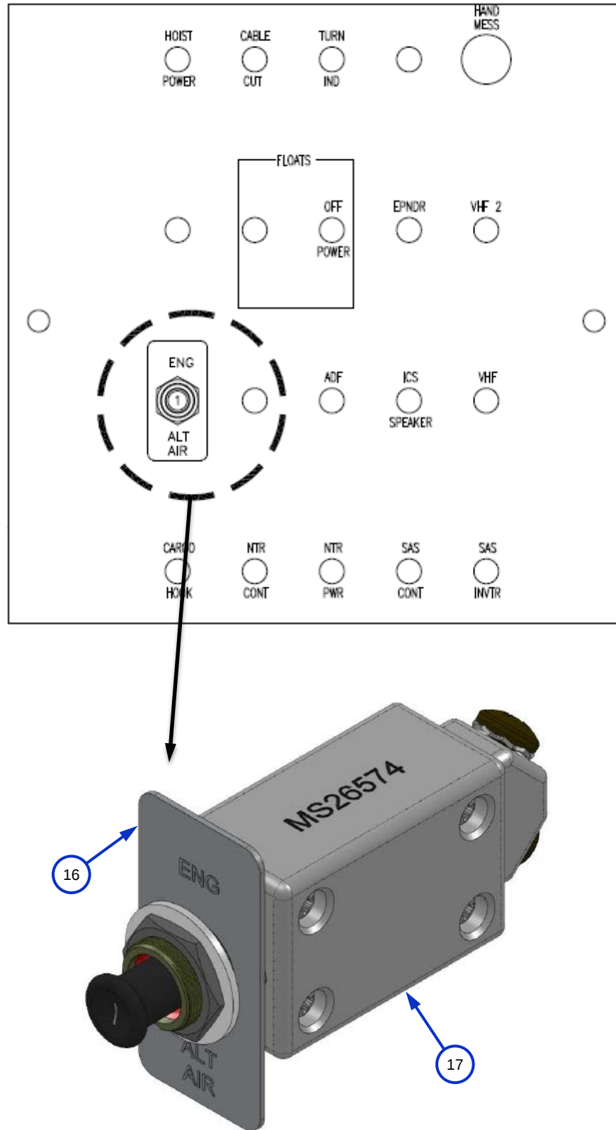
Figure 4-4: CIRCUIT BREAKER INSTALLATION (ON OVERHEAD PANEL)
