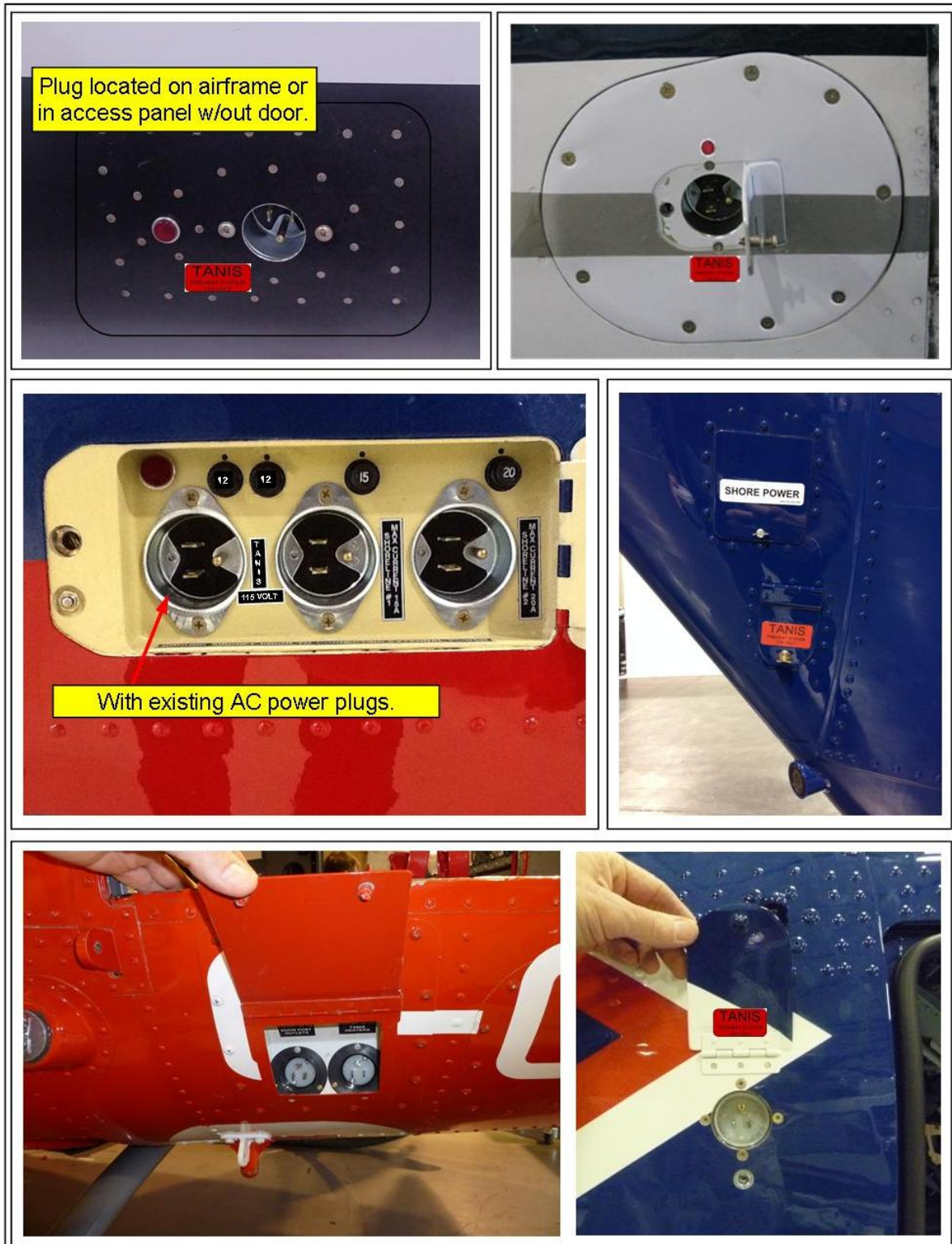
Figure 2 - Shore power plug, actual configuration may vary from depictions.
