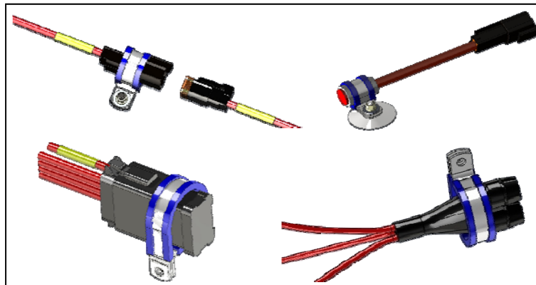
Figure 4 - Mounting options and clamp positions shown for connectors, indicator light, junction, and dual fused link.
