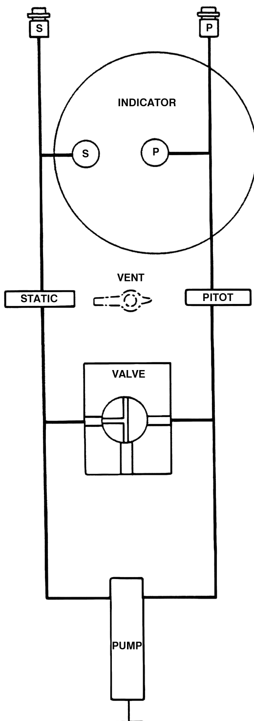
Ground Support Equipment – Instruments Figure 8 (Sheet 2 of 2)
