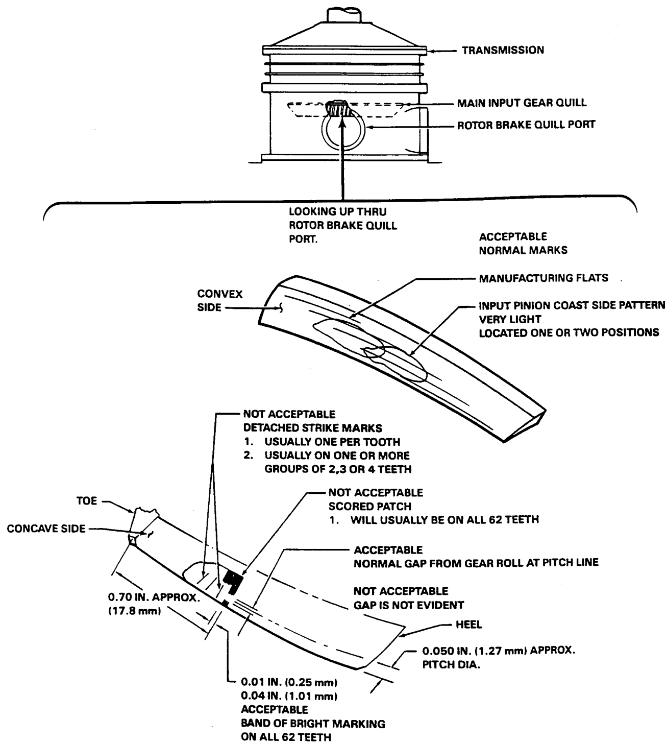
Figure 5-11. Spiral Bevel Gear Inspection (Sheet 1 of 3)
